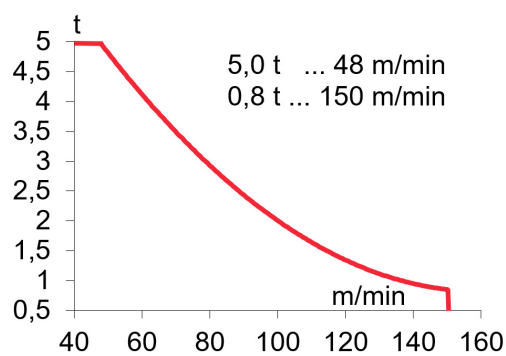
*EC60150VF 45 kW
