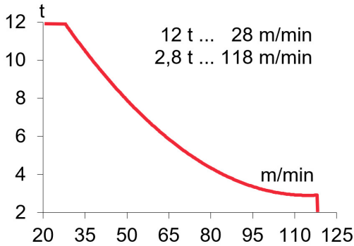
EC88115VF 65 kW
